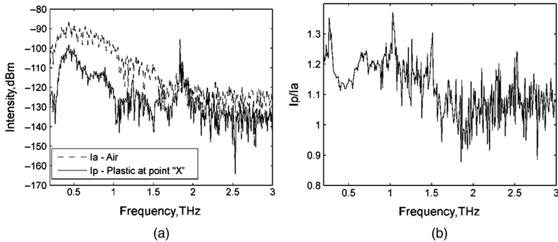
Fig. 3 The intensity of output signals for when the THz radiation passed through room air without the cuvette (la) and when THz radiation passed through both (a) room air and the cuvette at the point “X” (lp) and (b) the ratio of these signals.
